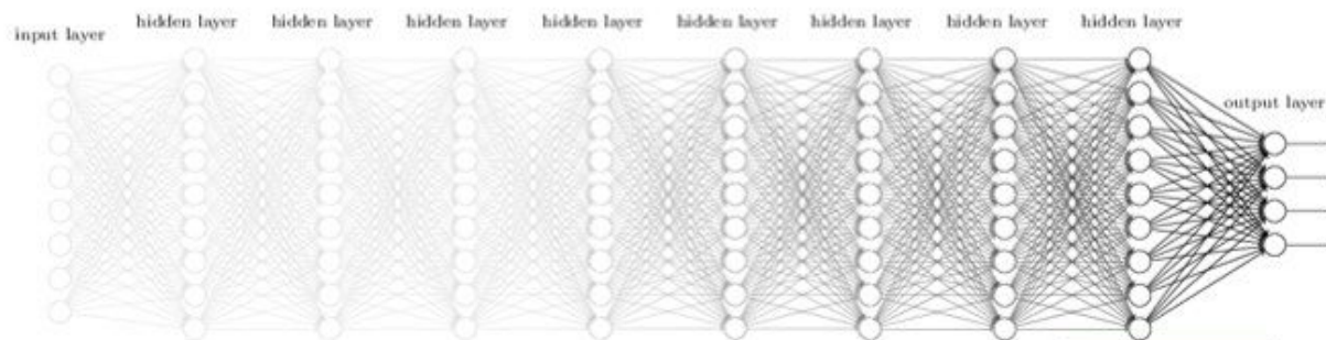
Vanishing Gradient
